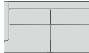
LA9180LL Englander Left Arm Loveseat Overall: W72 D42 H39 Inside: W68 D23 H19 Arm height: 36 SSeat height: 20 Two seat cushion, two back pillow Welt trim Nail trim available Standard finish: Antique Walnut
